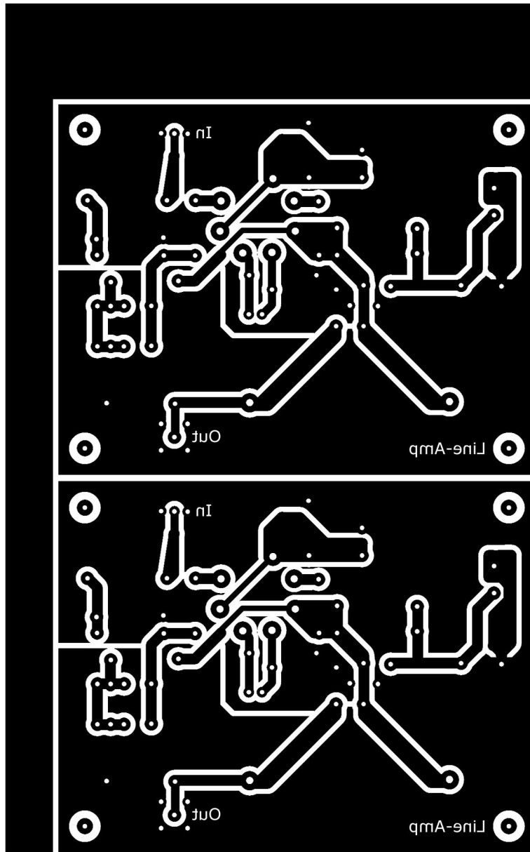
Platinenfilm Lineamp
